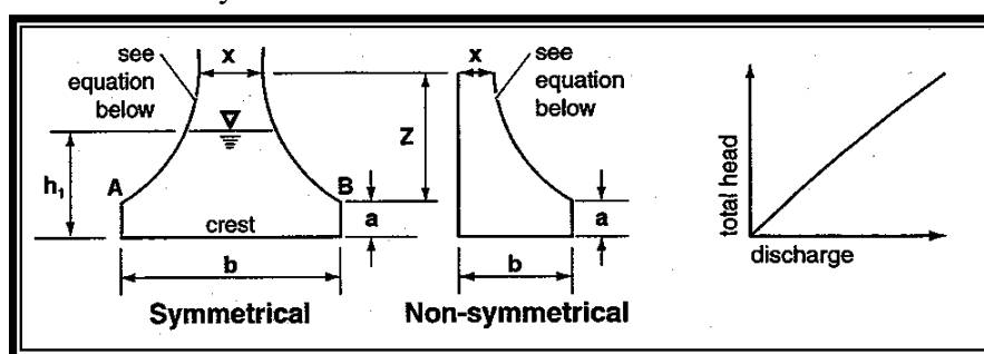
Figure 3.17. Sutro Weir.
