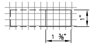
BLIND PICK NOTCH DETAIL
