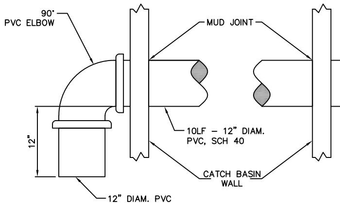
ELBOW DETAIL
