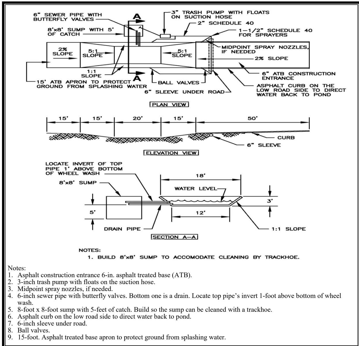
Figure 3.1. Wheel Wash.
