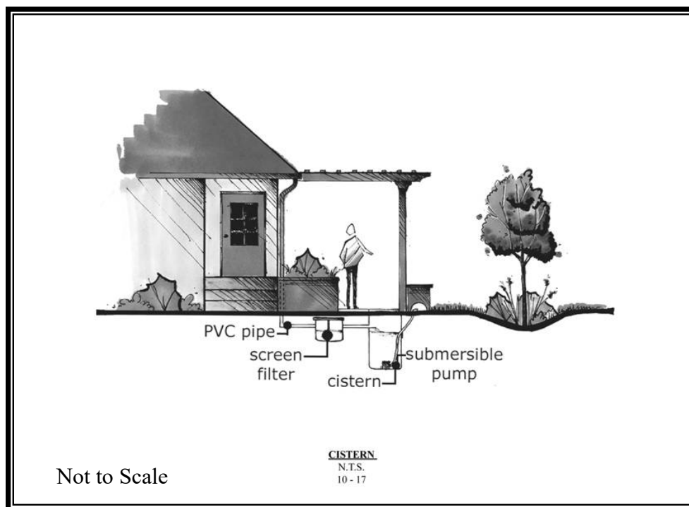
Figure 3.13. Cistern.
