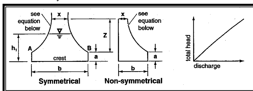
Figure 3.17. Sutro Weir.
