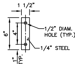
STEEL STRAP
