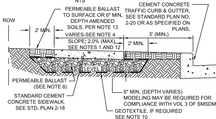
SIDEWALK WITH PLANTER STRIP SECTION
