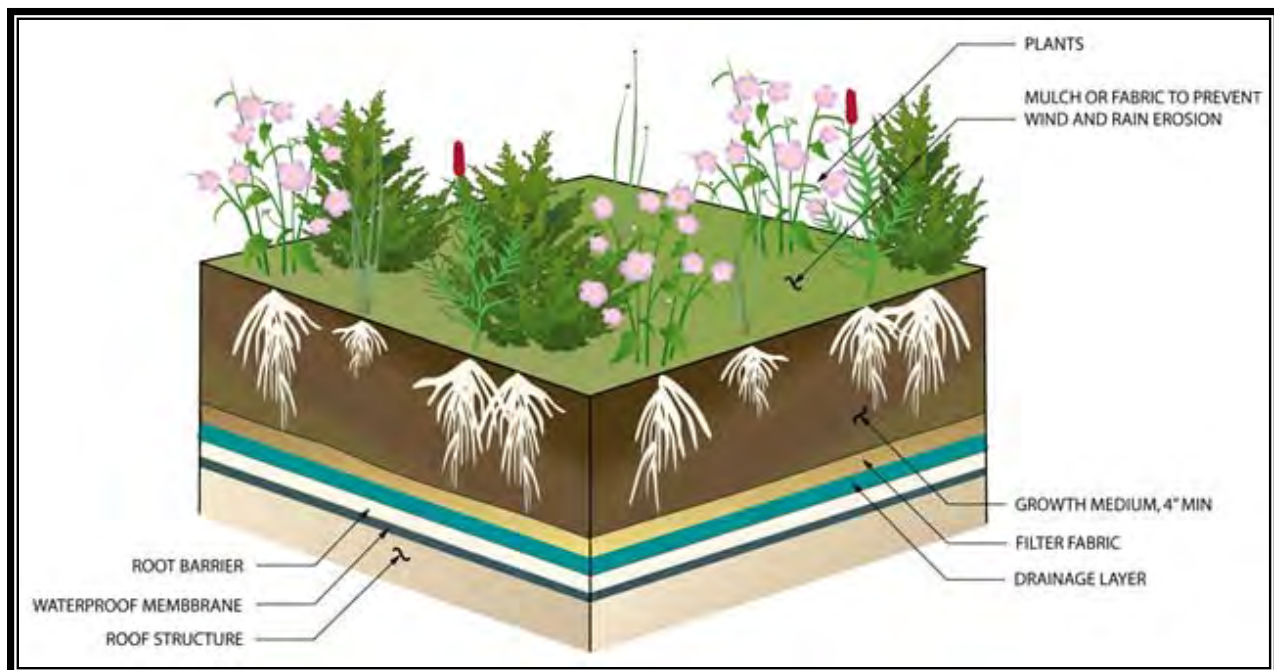
Figure 3.12. Vegetated Roof.
