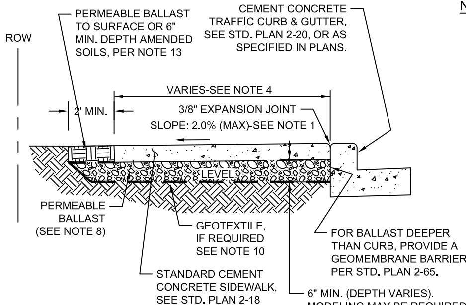
COMBINATION WALK SECTION
