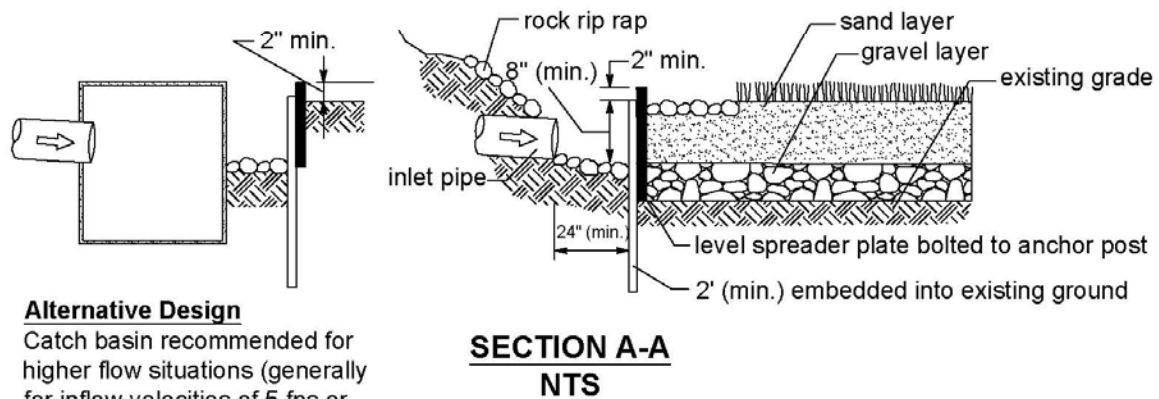
Figure 4.3. Flow Spreader Option A: Anchored Plate.
