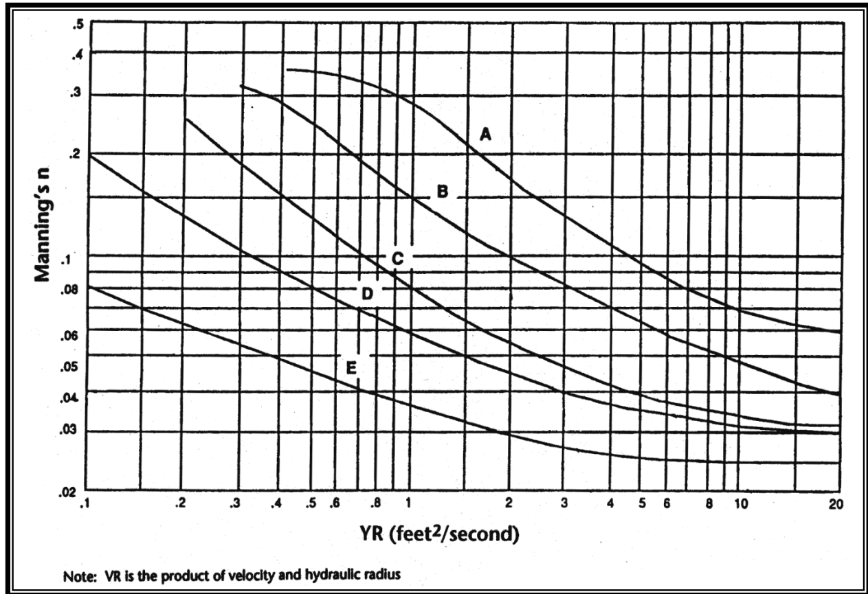
Figure 8.7. The Relationship of Manning's n with VR for Various Degrees of Flow Retardance (A-E).
