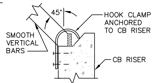
DETAIL HOOK CLAMP
