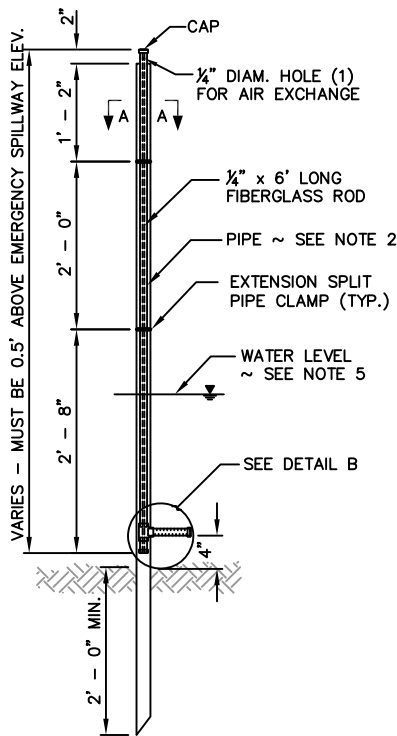
CREST GAGE
