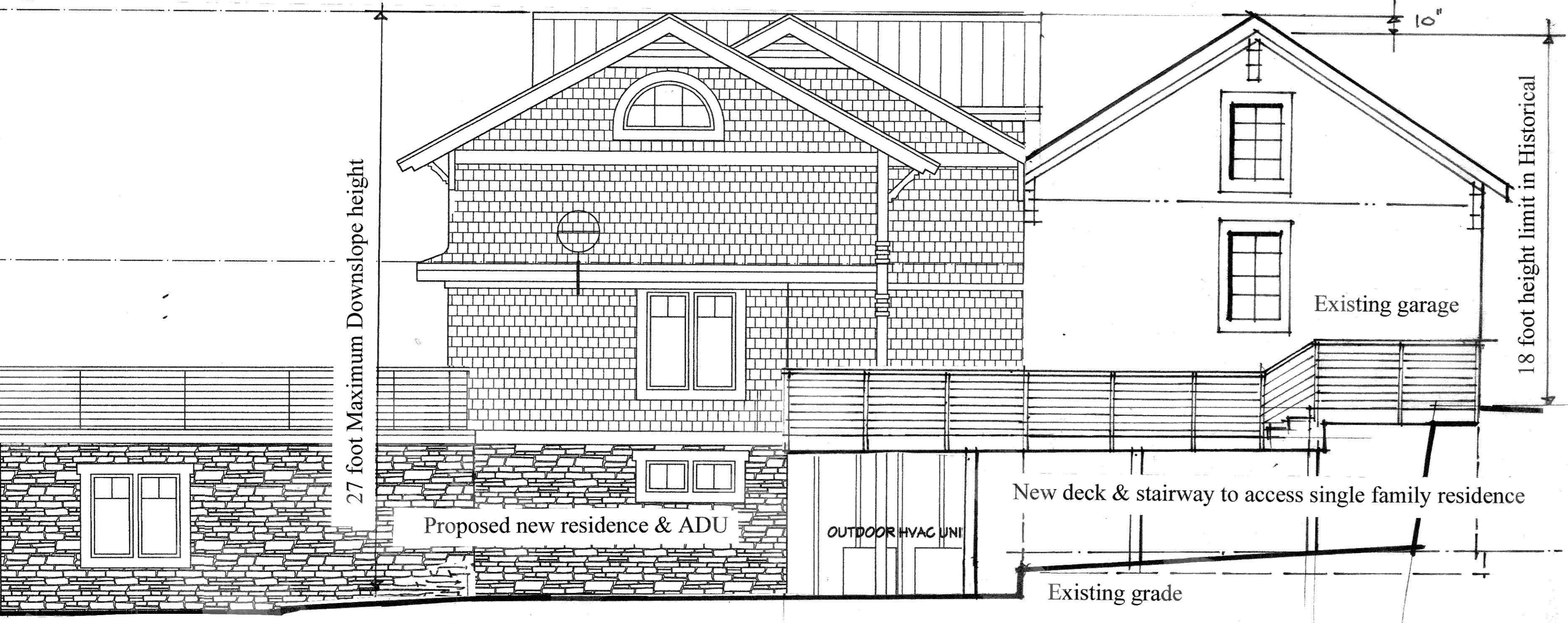
West Elevation
