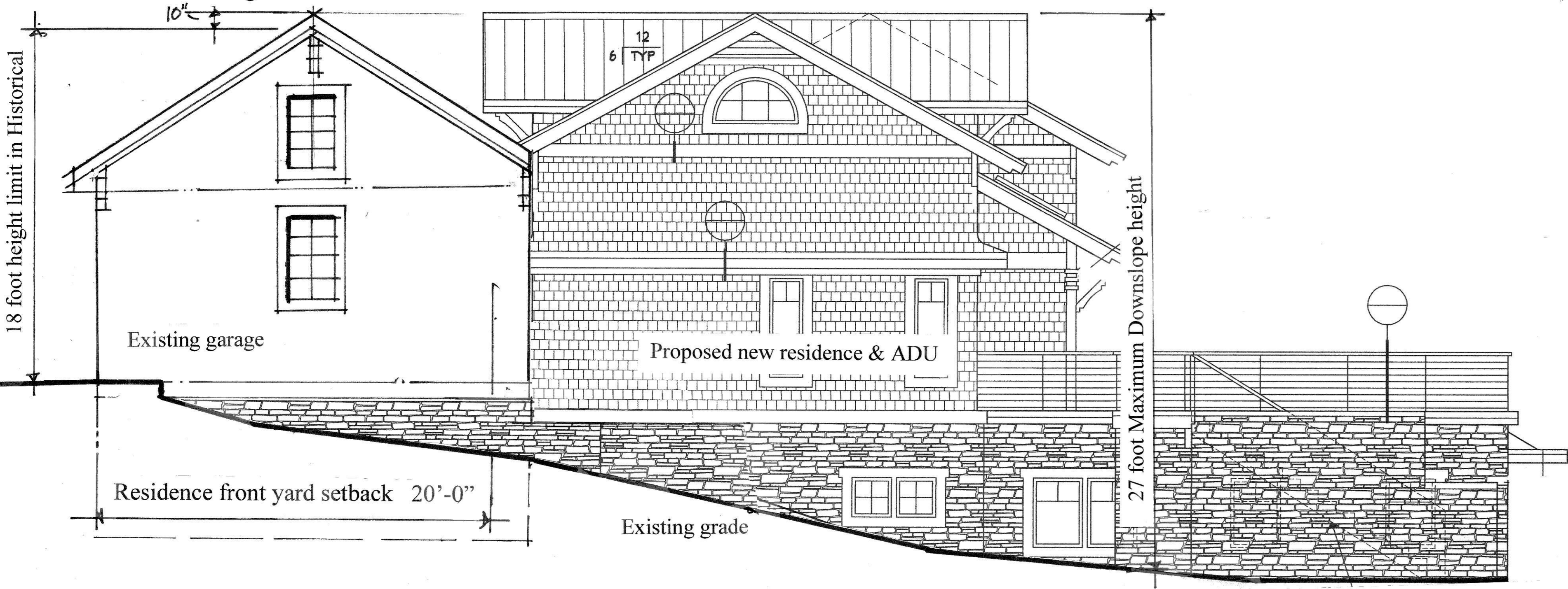
East Elevation
