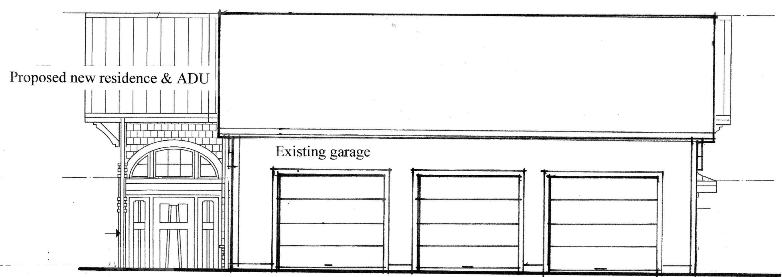
South Elevation
